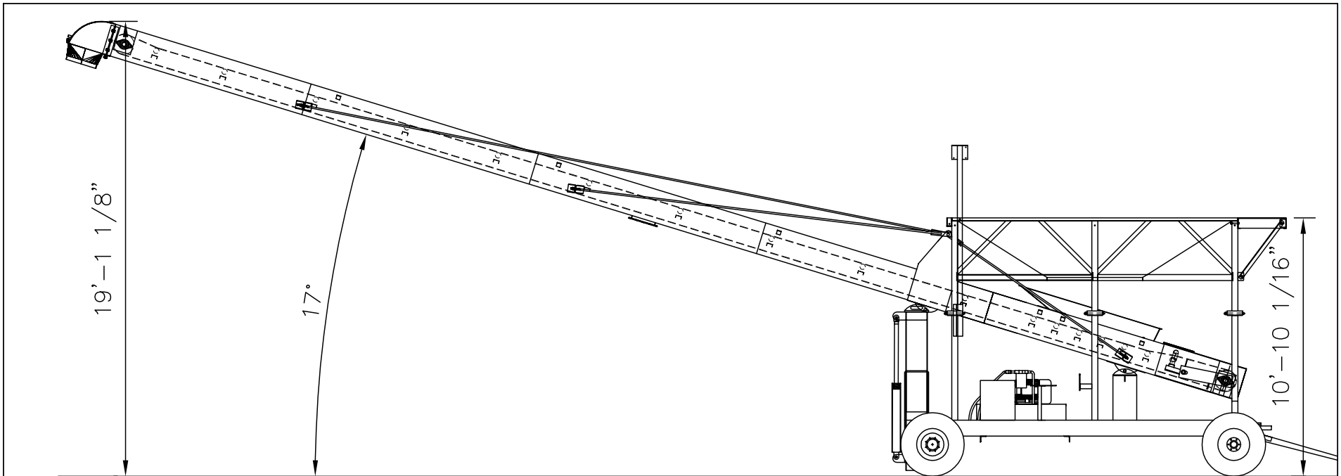
CONVEYOR WITH CYLINDER EXTENDED
